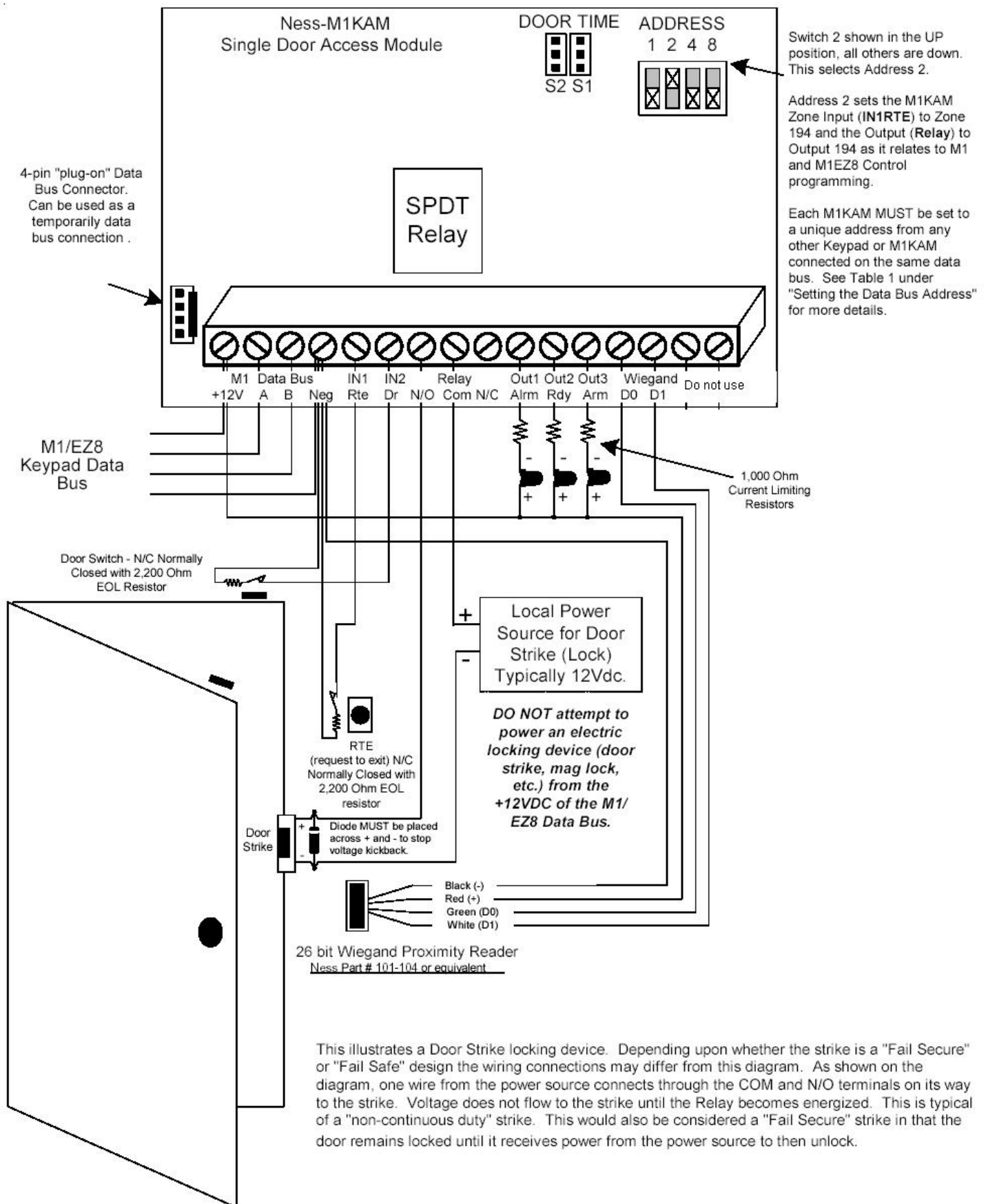
Hookup Diagram for Ness-M1KAM Single Door Access Module
